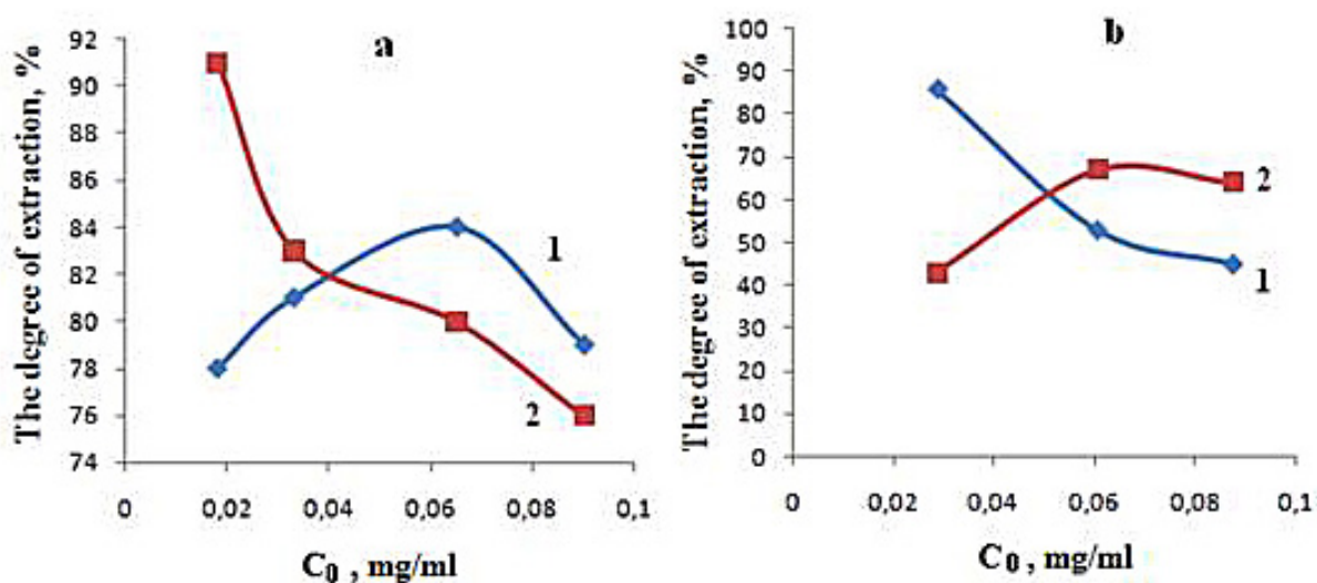
Figure 7. The degree of extraction of nickel ions on natural kaolin (a) and montmorillonite clay (b) in the Na-orm (1), OH-form (2)
