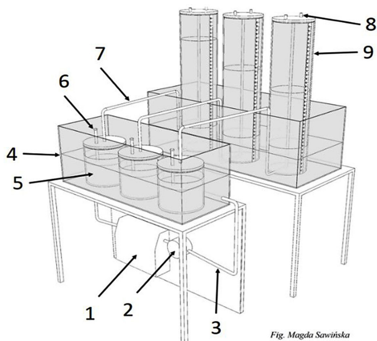
Fig. 2. Scheme of biofermenter for biogas production research (3-chamber section)
