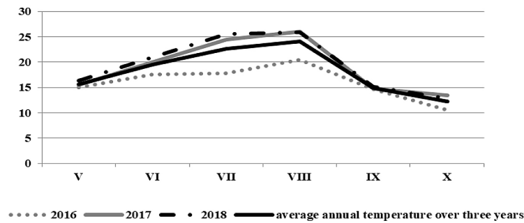
Fig. 1. Average monthly temperatures from May to October in 2016–2018 in Łańcut [°C]
