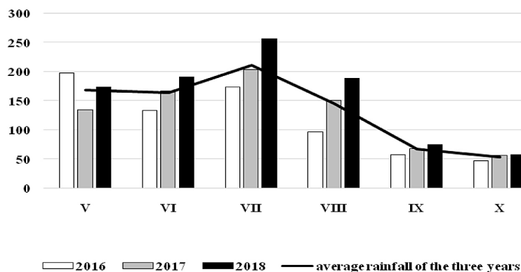
Fig. 2. Average monthly rainfall from May to October in 2016–2018 in Łańcut [mm]
