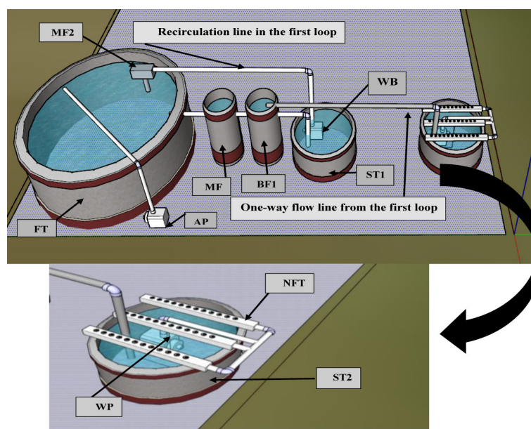
Figure 1. A schematic illustration of NFT of original DRAPS was used in Universiti Putra Malaysia. (AP) Air pump, (FT) fish tank, (MF) mechanical filter, (BF) biological filter, (ST1) sump tank 1, (WP) water pump, (MF2) mechanical filter 2. The second loop is composed; (NFT) hydroponics unit (NFT trials), (ST2) sump tank 2, (WP) water pump
