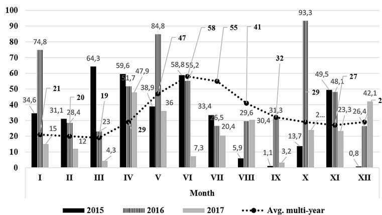
Fig. 2. The amount of precipitation in the years of the research in comparison with the average multi-year indices, mm
