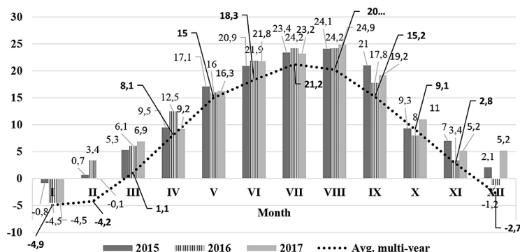
Fig. 1. The average monthly air temperature in the years of the research in comparison with the average multi-year indices, °C
