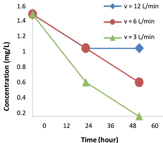
Figure 3. Effect of flow rate to the adsorption of NH 3 at the end of harvesting
