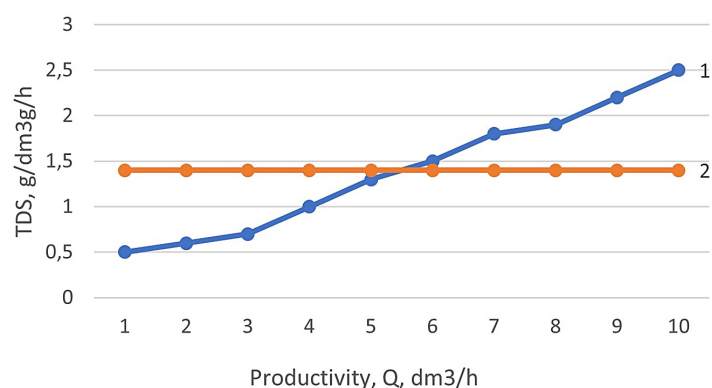
Figure 7. Productivity of CWTP from the total amount of dissolved substances TDS (Total dissolved solids)
