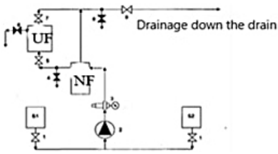
Figure 4. Schematic diagram of the operation of the UFU and NFU unit.
