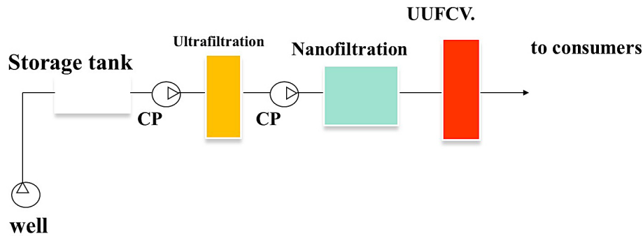
Figure 1. Technological block diagram of a combined water treatment plant (CWTP)
