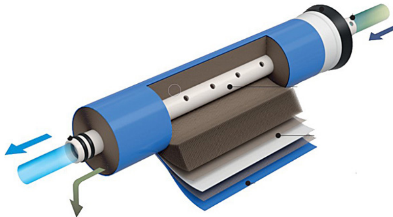
Figure 5. Construction and materials of membranes of ultra and nano filtration module
