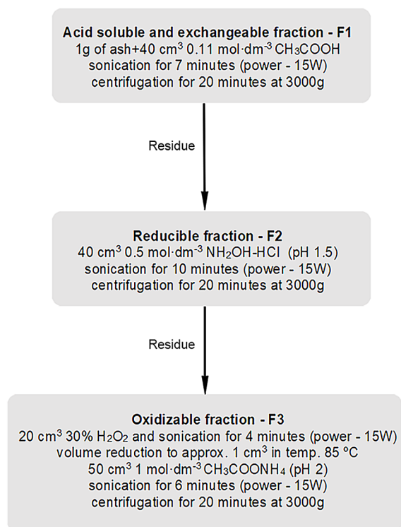
Figure 1. The BCR sequential extraction scheme
