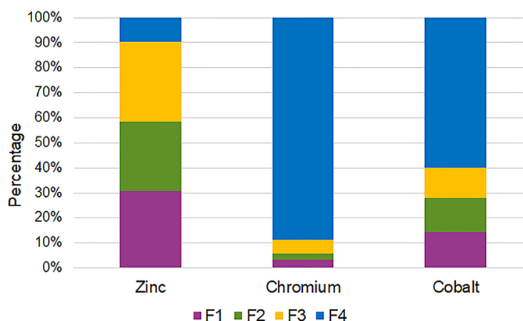
Figure 2. Fractional composition of Zn, Cr and Co in MSWI bottom ash
