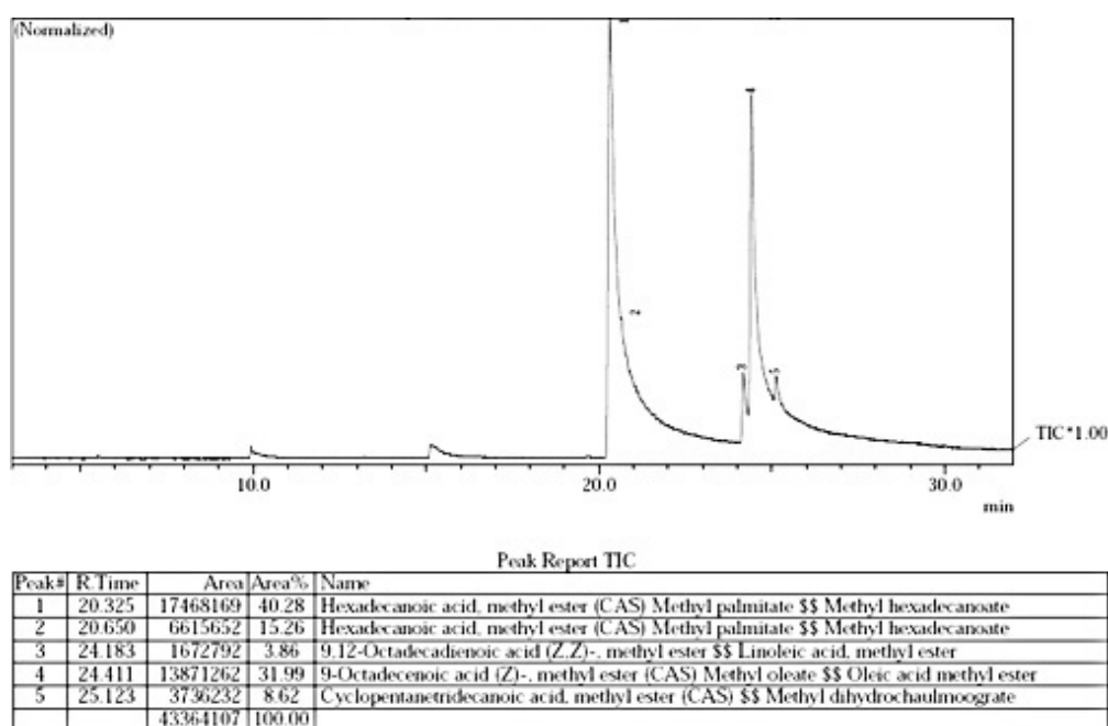
Figure 6. GC-MS biodiesel analysis
