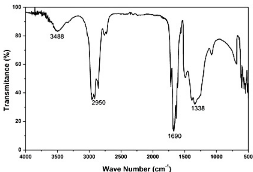
Figure 3. Results of FTIR analysis of catalyst
