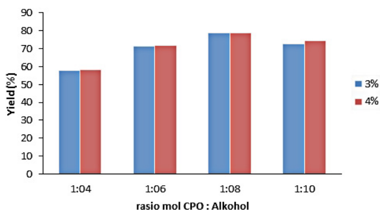
Figure 1. Biodiesel yield without the addition of co-solvent with two variations of catalyst weight
