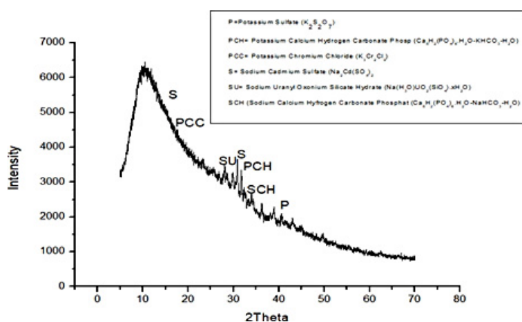
Figure 4. Results of XRD analysis of catalyst
