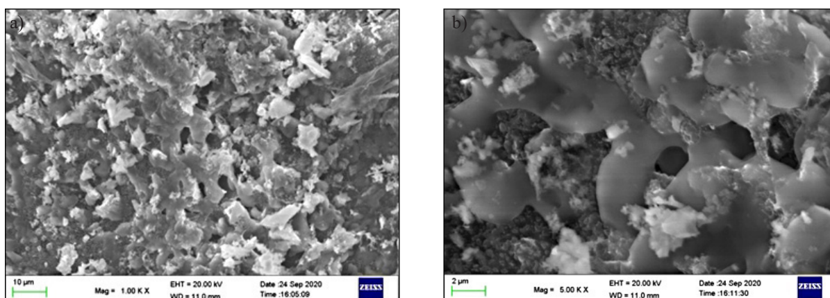
Figure 5. SEM of catalyst with magnification (a) 1000× (b) 5000×
