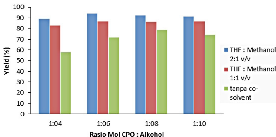
Figure 2. Biodiesel yield with a ratio of THF: Methanol 1:1 and 2:1 and without the addition of co-solvent with a catalyst weight of 4%
