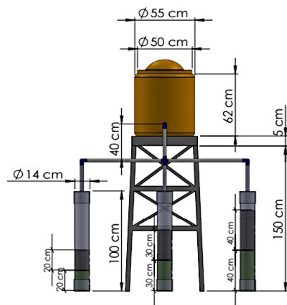
Figure 1. Filter reactor
