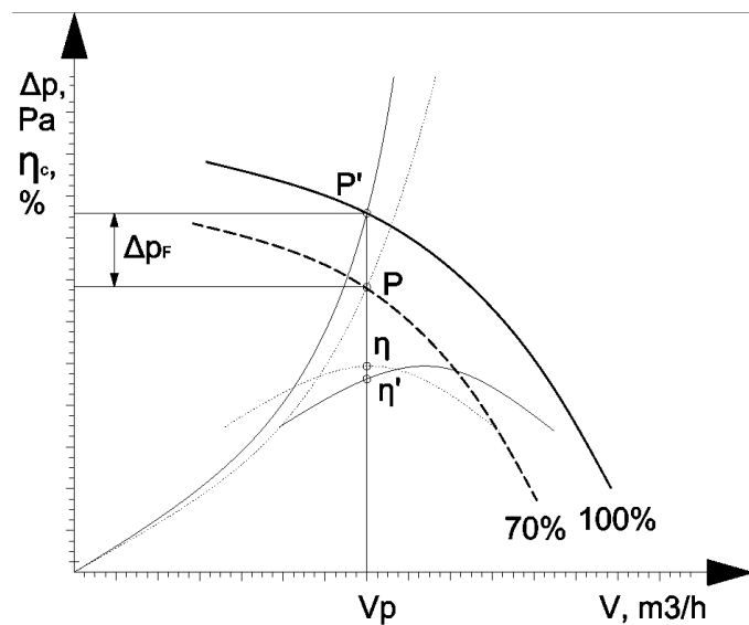
Figure 5.. Change of fan operation state after increasing of filters pressure drop
