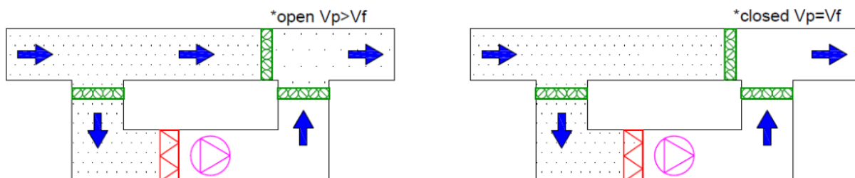
Figure 2. The idea of a cleaning device in the by-pass duct, based on [3a]
