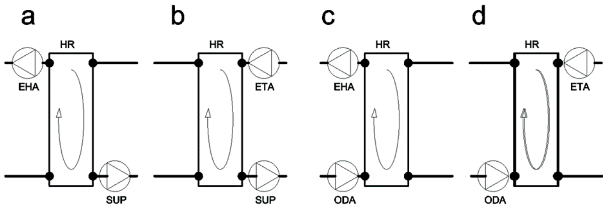
Figure 4. Possible configurations of the fans in relation to the heat recovery system in the air handling unit
