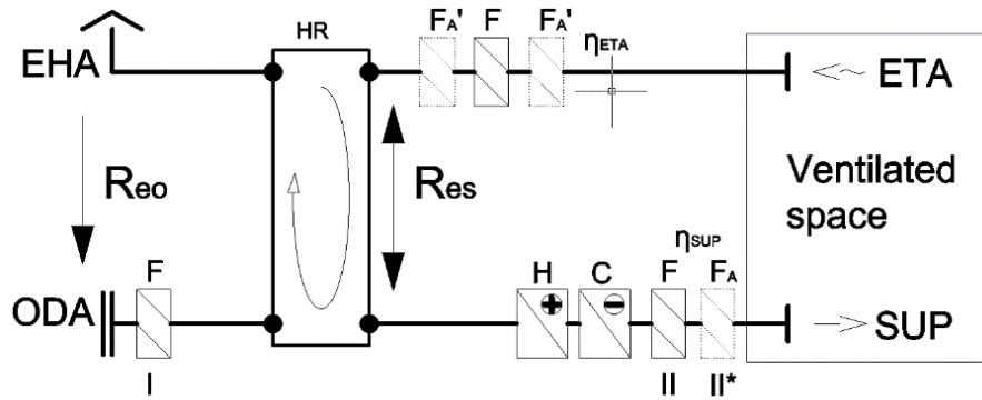
Figure 3. Diagram of the ventilation device and the locations of additional air purification facilities under consideration, FA – additional filter on the supply air, FA’ – additional filter on the extract air, Res – air flow of leak between extract and supply air and ventilating air flow ratio, Reo – air flow of leak between air intake and air discharge and ventilating air flow, EHA – exhaust air, ETA – extract air, ODA – outdoor air, SUP – supply air, \eta_{SUP} – efficiency of the additional filter on the supply air, \eta_{ETA} – efficiency of the additional filter on the extract air
