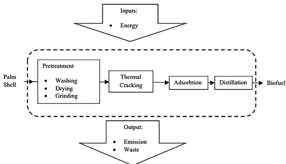
Figure 2. Boundary system of biofuel production process
