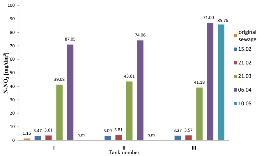
Figure 6. Changes in nitrates concentration
