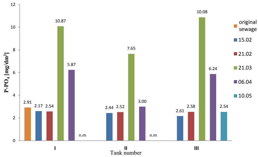
Figure 5. Changes in phosphates concentration
