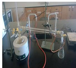
Fig.7: Distillation process
