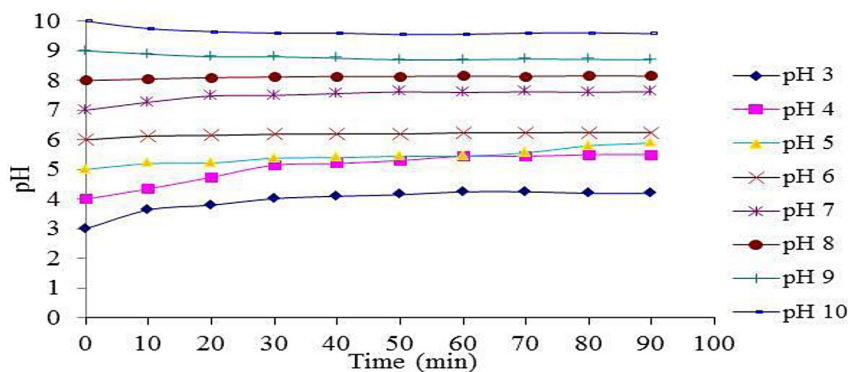
Figure 3. Changing in pH during the indirect electrochemical oxidation of restaurant wastewater (initial pH 3–10)
