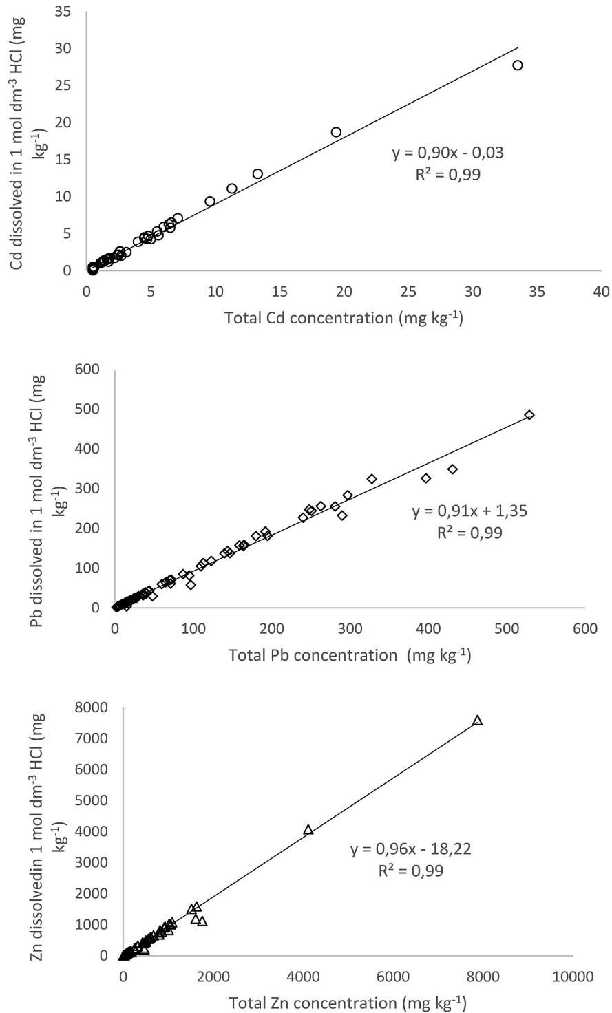
Figure 2. Relationship between total content of Cd, Pb and Zn and their bioaccessible fractions extracted with 1 mol dm -3 HCl
