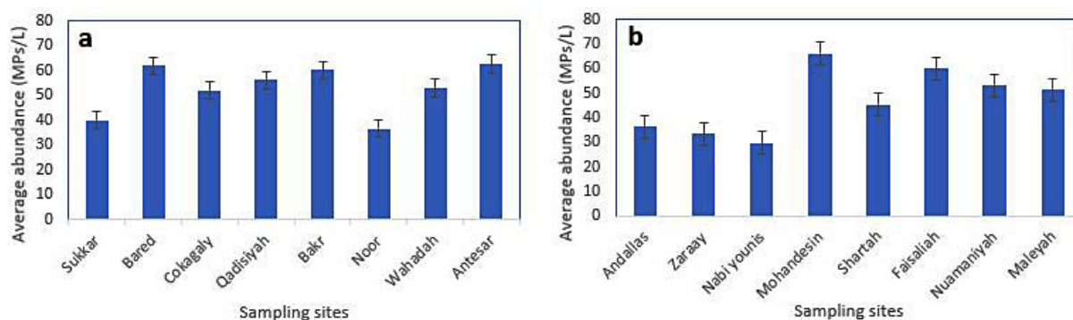
Figure 3. Average abundance of microplastics in selected districts of (a) AJ-WDN and (b) AQ-WDN
