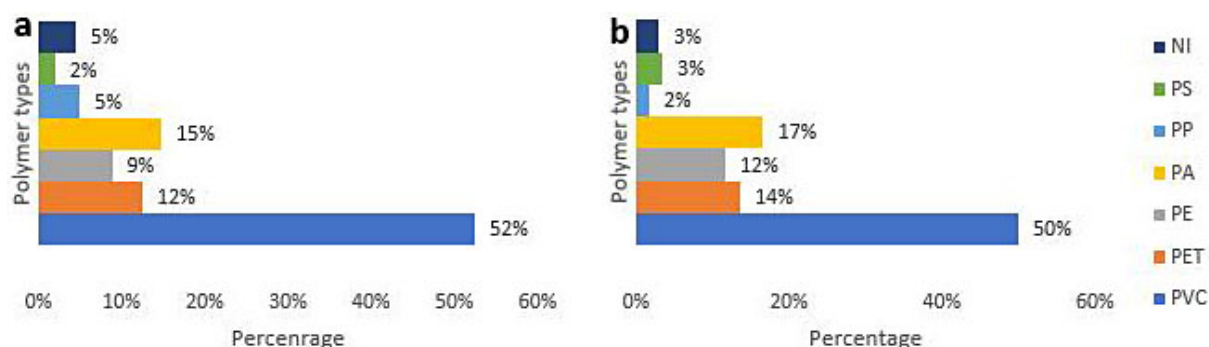
Figure 7. Polymer types percentage of microplastics in selected districts of (a) AJ-WDN and (b) AQ-WDN. Polymer identification: PVC – polyvinyl chloride, PA – polyamide, PET – polyethylene terephthalate, PE – polyethylene, PS – polystyrene, NI – non identified polymer
