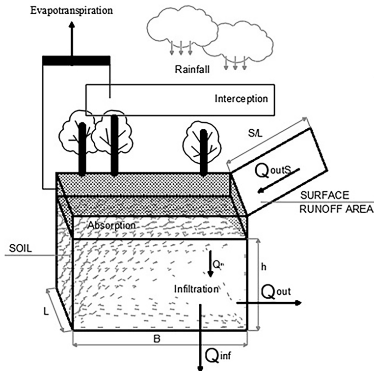
Figure 4. Schematic representation of the infiltration system
