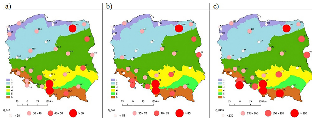
Figure 7. The size of the regulated runoff from the infiltration trench considering the sealing of the urban catchment: a) small, b) medium, c) high
