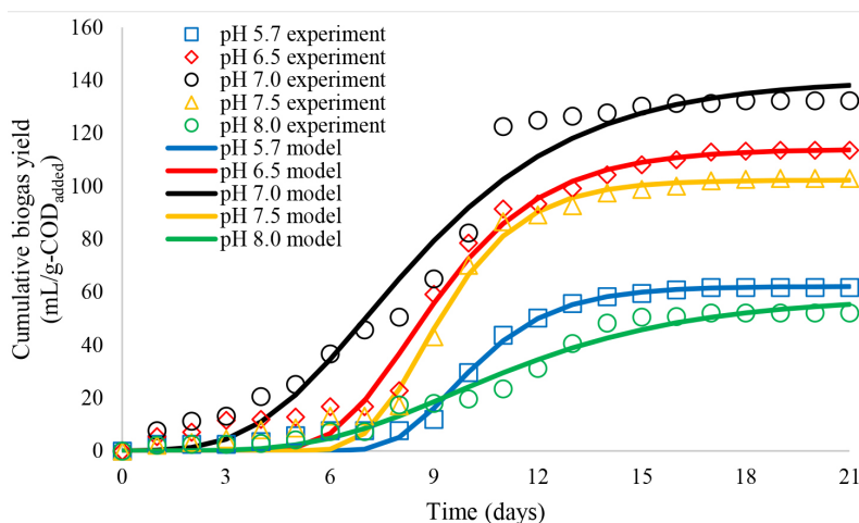
Figure 6. Plotting results using the modified Gompertz model
