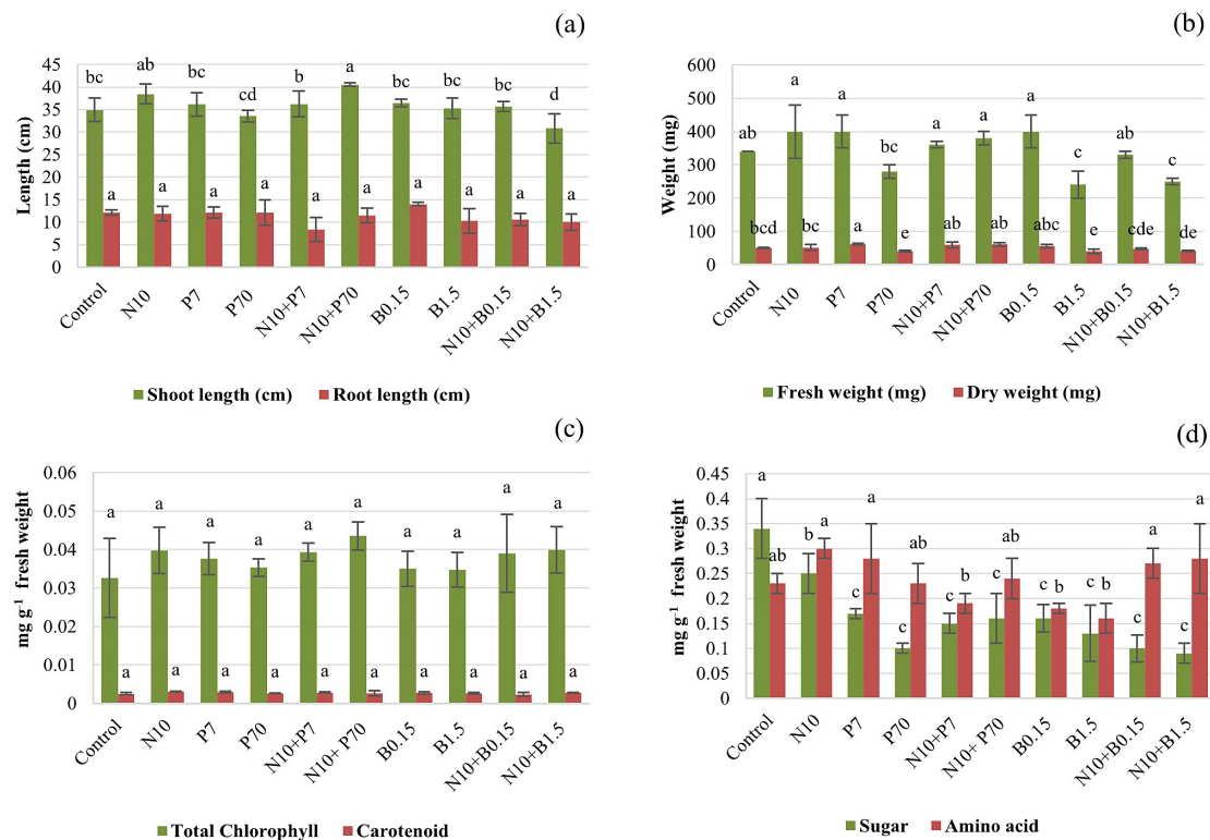
Figure 4. Effects of Nostoc sp. N1 (N), paraquat (P), and butachlor (B) on the physical and biochemical parameters of rice seedlings aged 21 days: (a) shoot length and root length, (b) fresh weight and dry weight, (c) total chlorophyll and carotenoid contents, (d) sugar and amino acid contents. Treatments: Control (no herbicide, no Nostoc ); N10 ( Nostoc sp. N1 at 10 g kg -1 ); P7 (paraquat at 7 mg kg -1 ); P70 (paraquat at 70 mg kg -1 ); N10+P7 (combination); N10+P70 (combination); B0.15 (butachlor at 0.15 mg kg -1 ); B1.5 (butachlor at 1.5 mg kg -1 ); N10+B0.15 (combination); N10+B1.5 (combination). Values represent mean ± standard deviation (n=3). For each parameter, bars sharing the same lowercase letter are not significantly different (p ≤ 0.05, DMRT)
