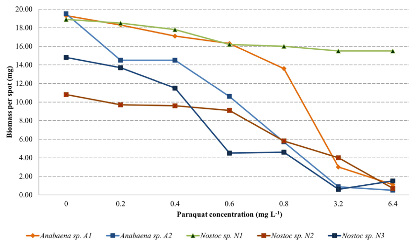
Figure 1. Dose-responses of cyanobacterial biomass to paraquat based on spot testing
