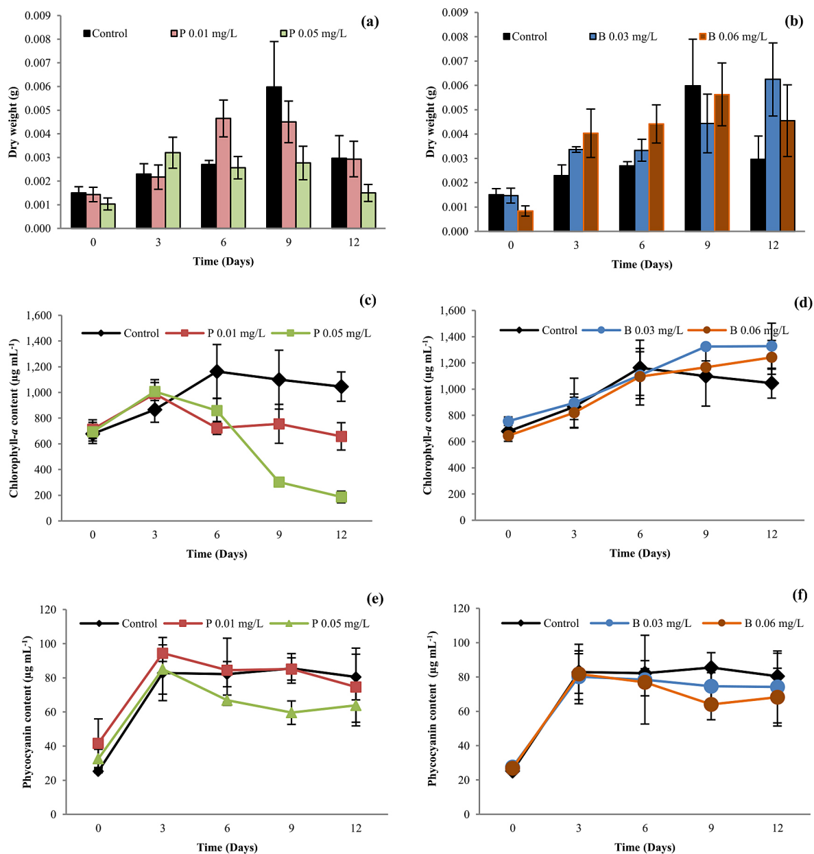
Figure 2. Toxicity of paraquat and butachlor on dry weight, chlorophyll, and phycocyanin contents of Nostoc sp. N1 : (a) Dry weight in response to paraquat, (b) Dry weight in response to butachlor, (c) Chlorophyll-a content in response to paraquat, (d) Chlorophyll-a content in response to butachlor, (e) Phycocyanin content in response to paraquat, and (f) Phycocyanin content in response to butachlor. Treatments: Control (no herbicide); P 0.01 (0.01 mg L -1 paraquat); P 0.05 (0.05 mg L -1 paraquat); B 0.03 (0.03 mg L -1 butachlor); B 0.06 (0.06 mg L -1 butachlor). Values represent mean ± standard deviation (n=3)
