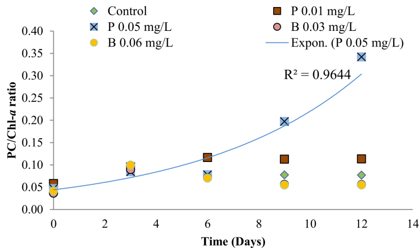
Figure 3. Phycocyanin-to-chlorophyll- a (PC/Chl- a ) ratio in Nostoc sp. N1 exposed to paraquat (P) and butachlor (B) over 12 days, showing exponential (Expon.) trendline for P 0.05 mg L -1 treatment ( R^2 = 0.9644 ), where points represent mean values ( n=3 )
