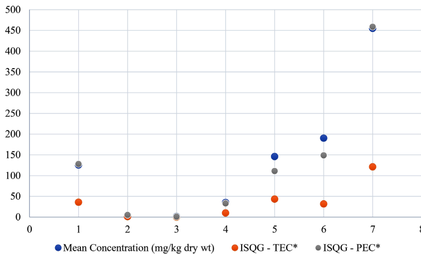
Figure 3. Heavy metal concentrations in river sediment compare with standards
