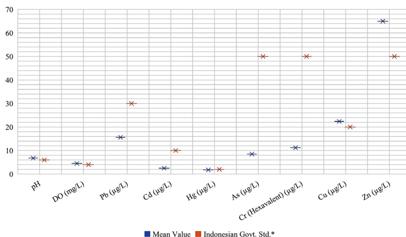
Figure 2. Physicochemical parameters and heavy metal concentrations in river water compare with standards
