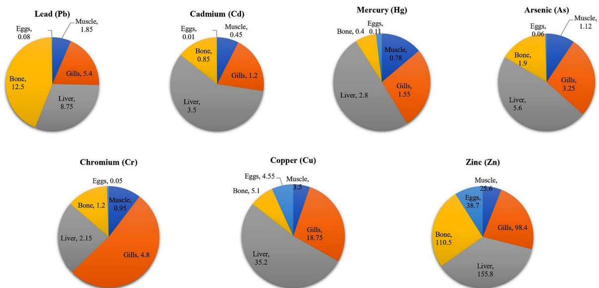
Figure 4. Comparative bioaccumulation of each heavy metal across tissues
